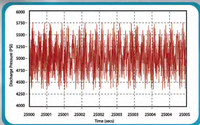
Without Dampener Pressure Variation - 1350 psi
