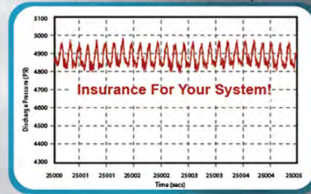
With Dampener Pressure Variation - 175 psi
