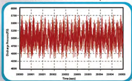
Without Dampener Pressure Variation - 1350 psi
